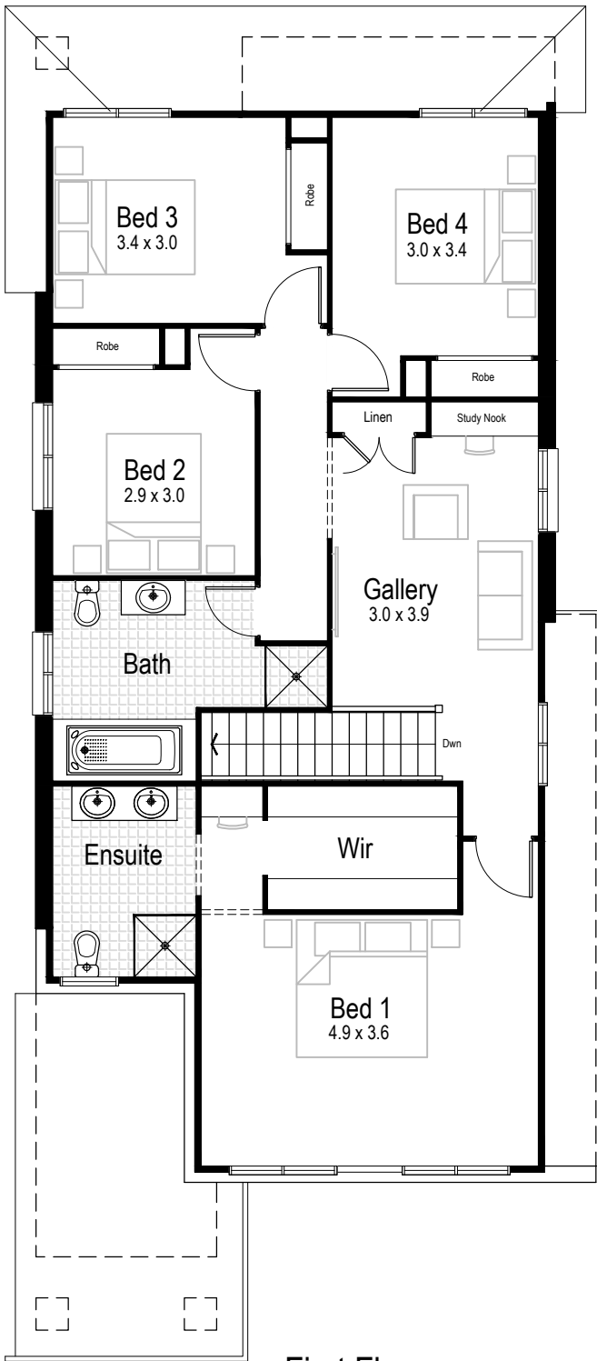
First Floor
