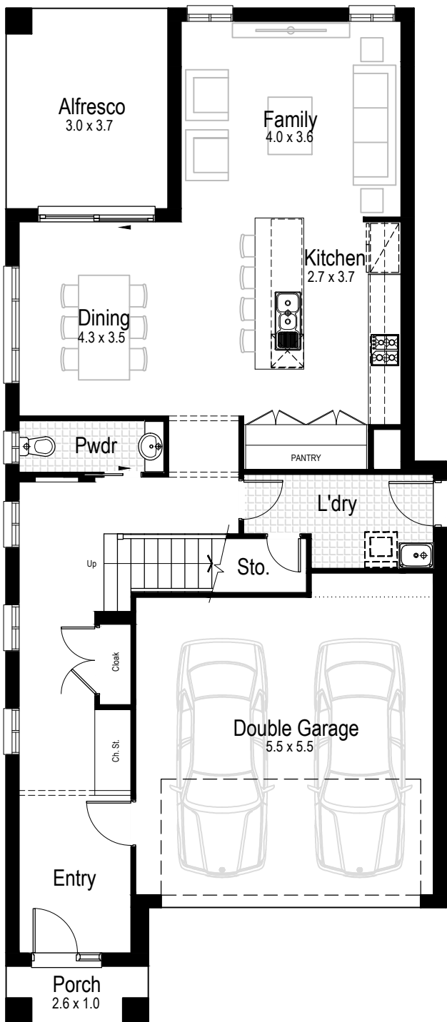
Ground Floor
